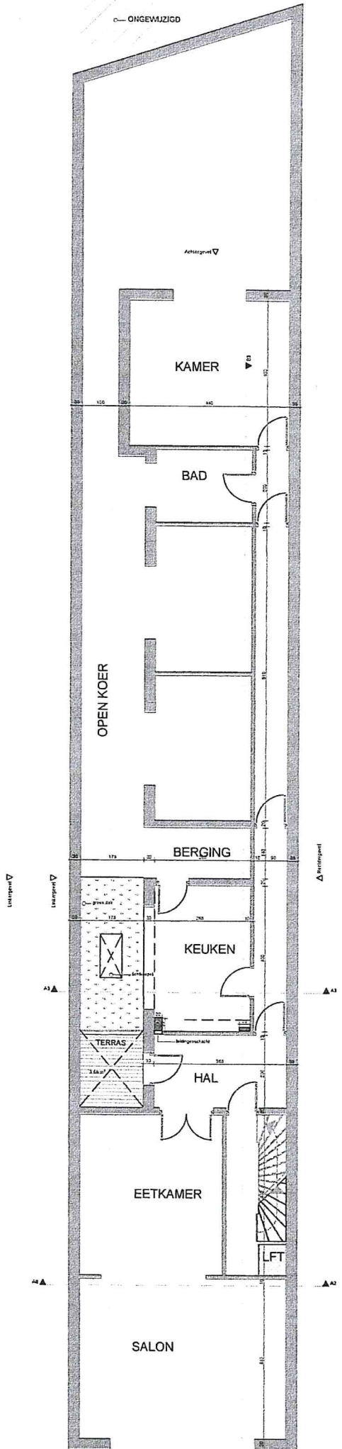
Begane grond 1/50
